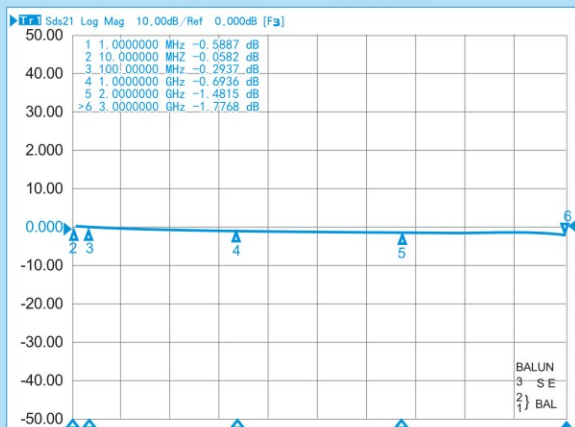
RFT4042G-1/1 插入损耗
