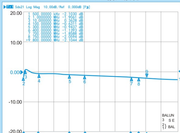
RFT4042A-1/1 插入损耗
