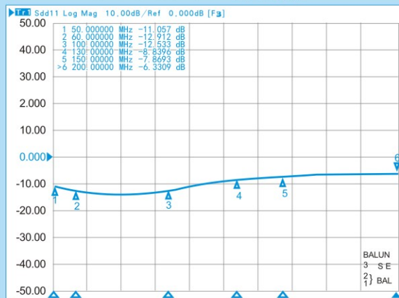
RFT4042A-1/4 返回损耗
