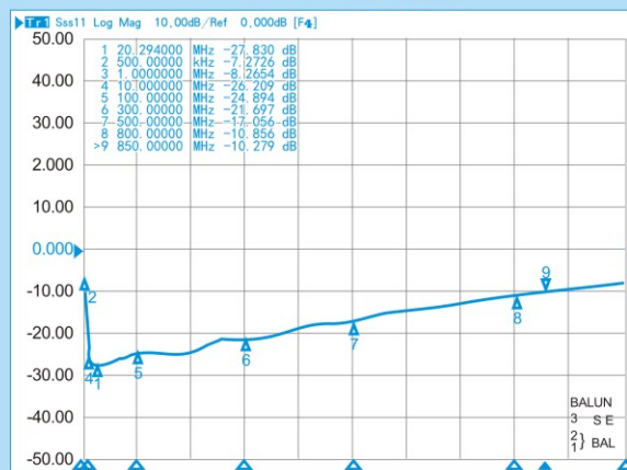
RFT4042A-4/1 返回损耗
