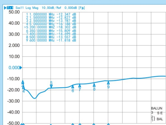
RFT4042C-1/1 返回损耗
