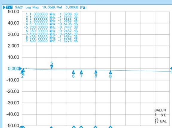
RFT4042C-1/1 插入损耗
